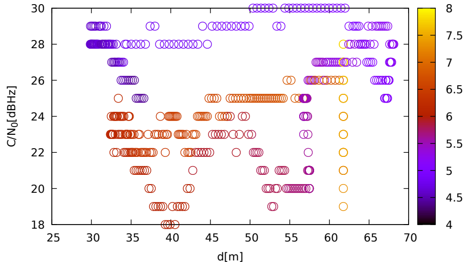
C/N 0 vs distance (ublox9 at C 1 for G31 at L2)
