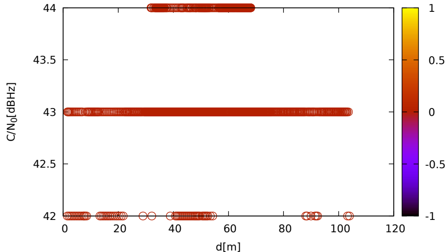
C/N 0 vs distance (ublox9 at C 1 for R07 at L2)
