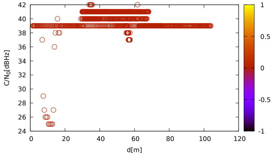
C/N 0 vs distance (ublox9 at C 1 for R08 at L2)
