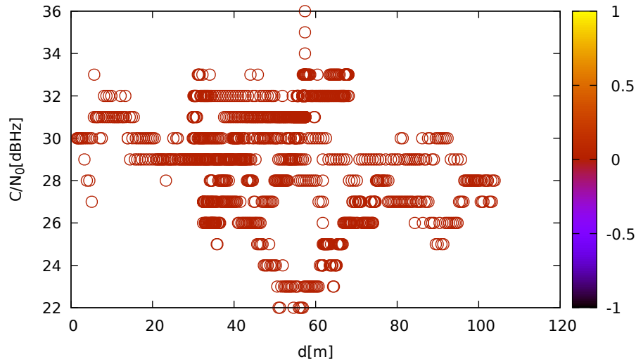
C/N 0 vs distance (ublox9 at C 1 for R14 at L2)
