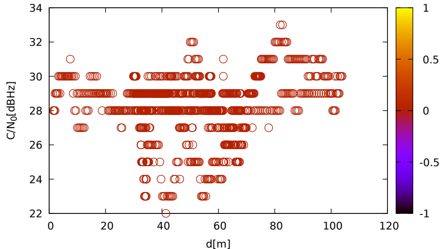
C/N 0 vs distance (ublox9 at C 1 for R15 at L2)
