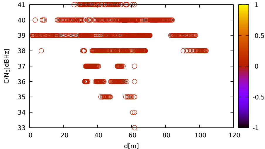
C/N 0 vs distance (ublox9 at C 1 for R21 at L2)
