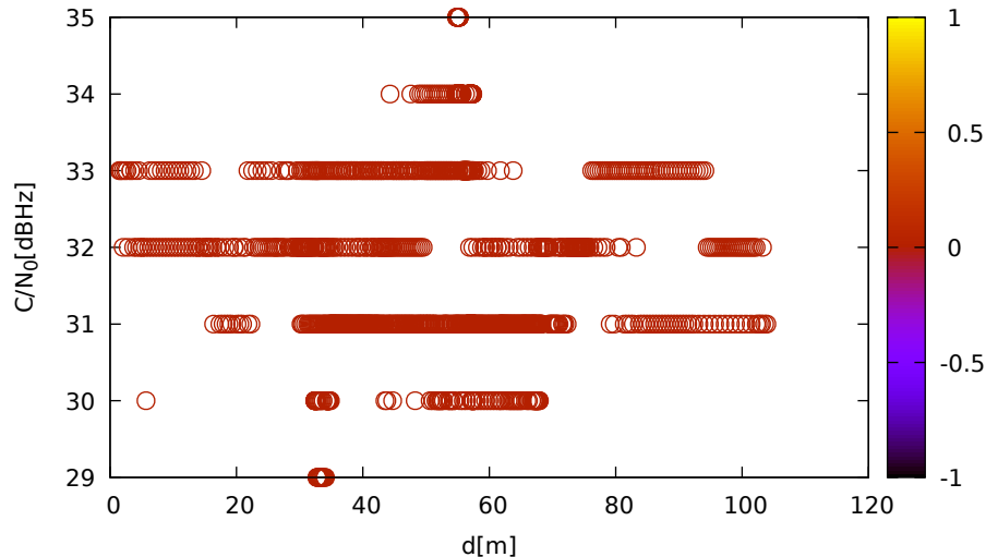
C/N 0 vs distance (ublox9 at C 1 for R23 at L2)
