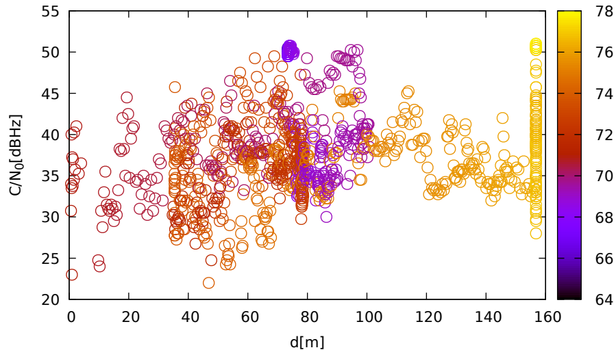
C/N 0 vs distance (JavadLSA at C 2 for G01 at L2)
