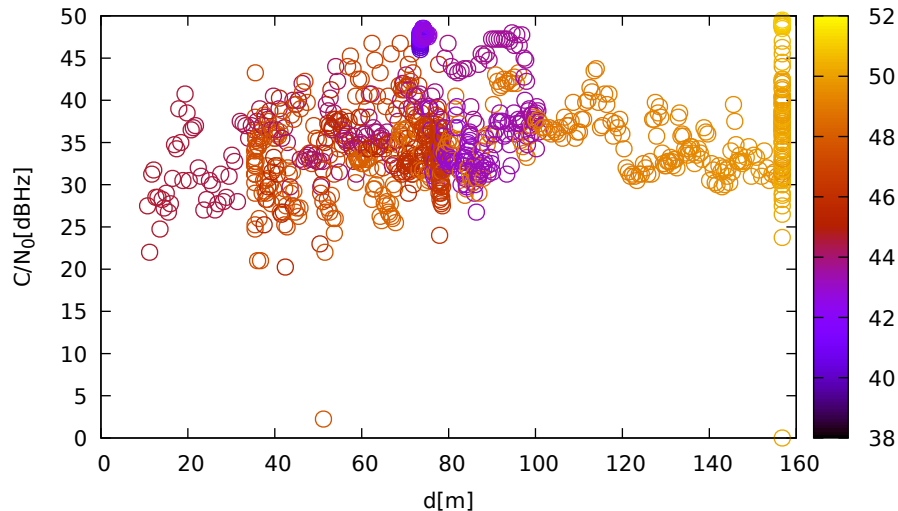
C/N 0 vs distance (JavadLSA at C 2 for G03 at L2)
