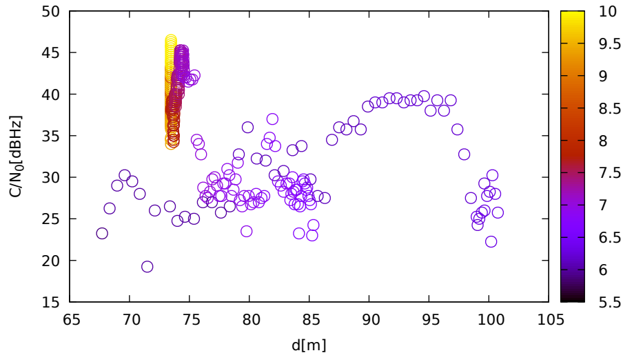
C/N 0 vs distance (JavadLSA at C 2 for G10 at L2)
