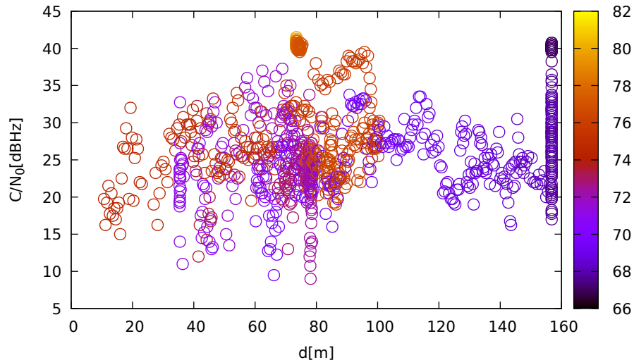
C/N 0 vs distance (JavadLSA at C 2 for G11 at L2)
