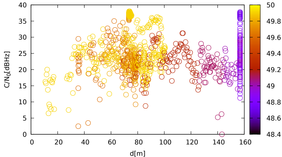
C/N 0 vs distance (JavadLSA at C 2 for G14 at L2)
