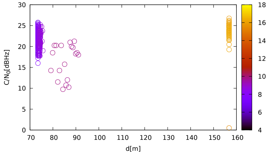
C/N 0 vs distance (JavadLSA at C 2 for G17 at L2)
