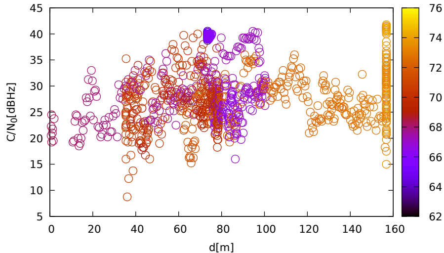
C/N 0 vs distance (JavadLSA at C 2 for G22 at L2)
