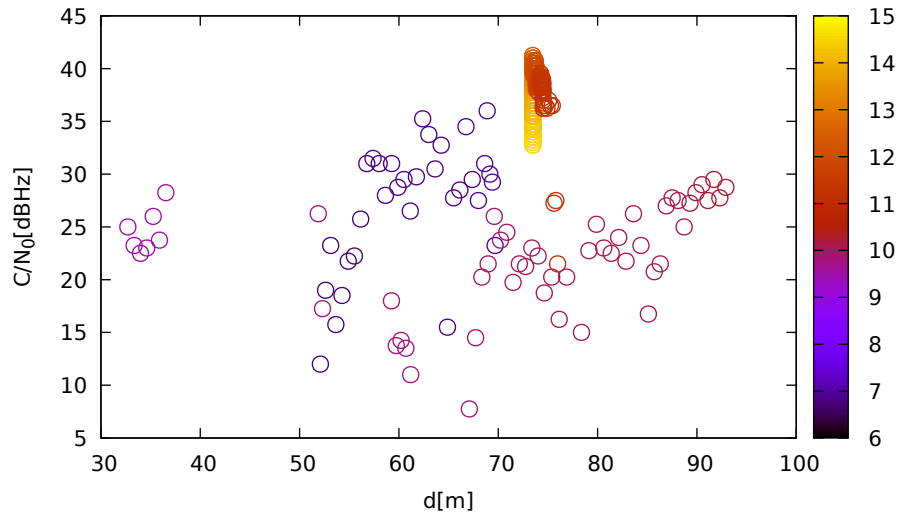
C/N 0 vs distance (JavadLSA at C 2 for G27 at L2)
