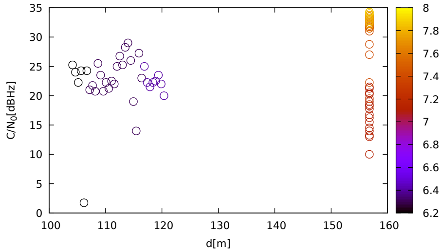
C/N 0 vs distance (JavadLSA at C 2 for G31 at L2)
