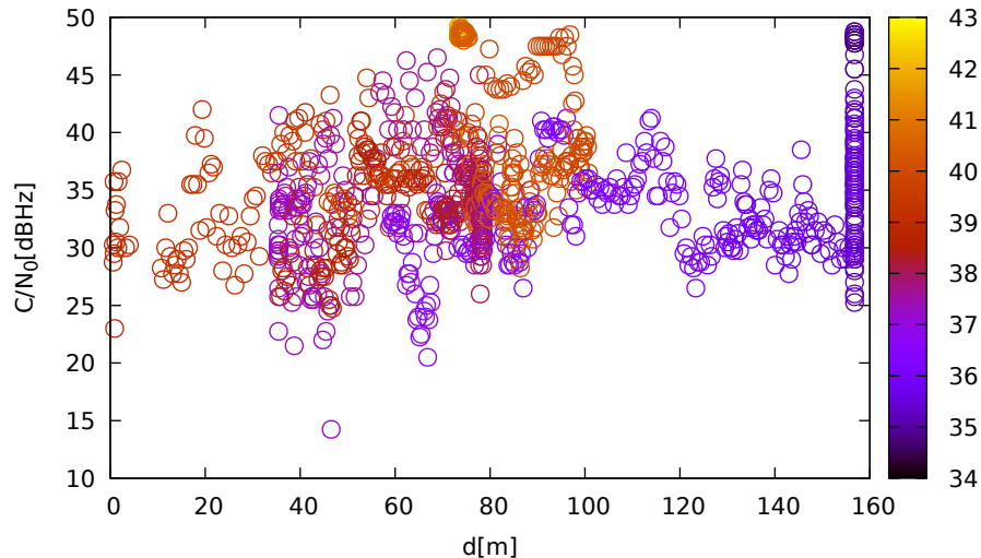
C/N 0 vs distance (JavadLSA at C 2 for G32 at L2)
