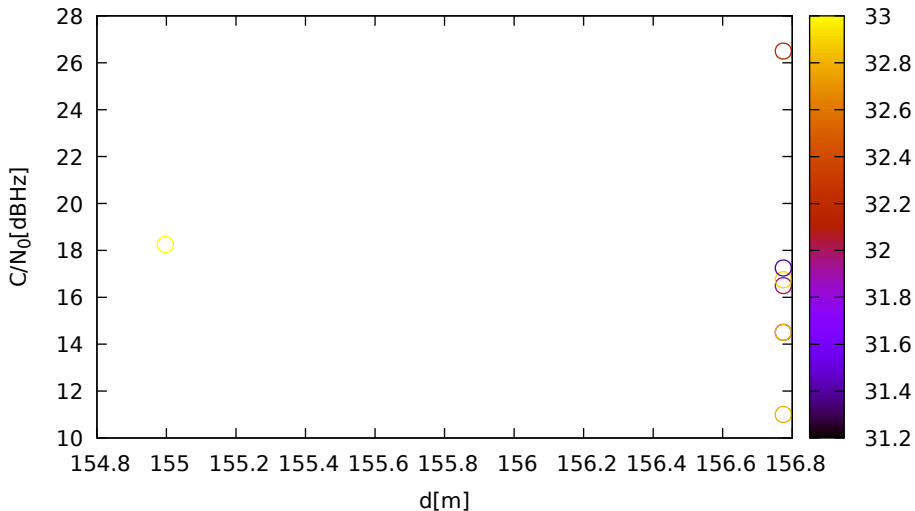
C/N 0 vs distance (JavadLSA at C 2 for R06 at L2)
