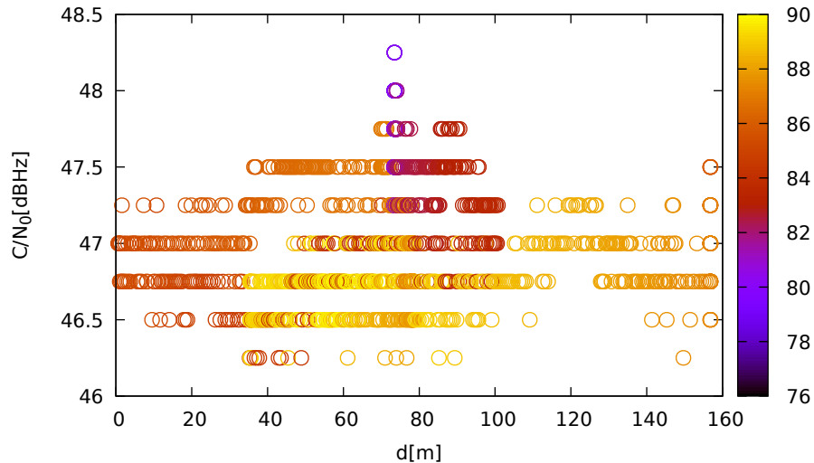
C/N 0 vs distance (JavadLSA at C 2 for R07 at L2)
