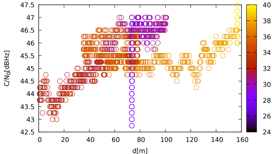
C/N 0 vs distance (JavadLSA at C 2 for R08 at L2)
