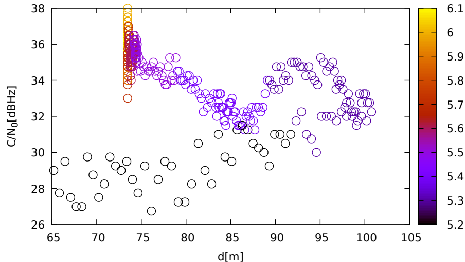
C/N 0 vs distance (JavadLSA at C 2 for R14 at L2)
