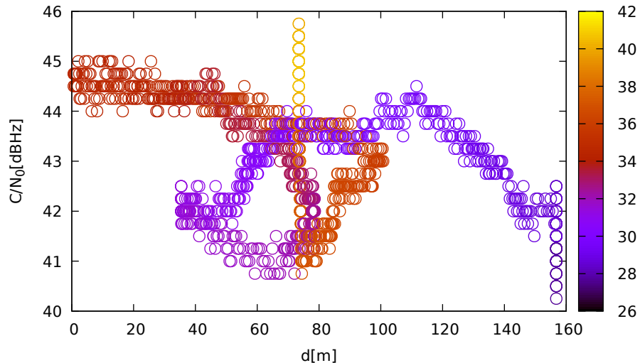
C/N 0 vs distance (JavadLSA at C 2 for R21 at L2)
