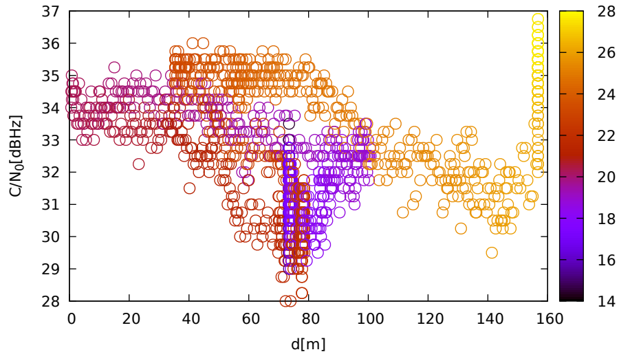
C/N 0 vs distance (JavadLSA at C 2 for R23 at L2)
