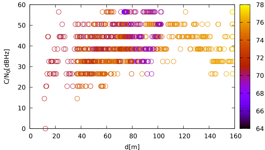
C/N 0 vs distance (LeicaGS15 at C 2 for G01 at L2)
