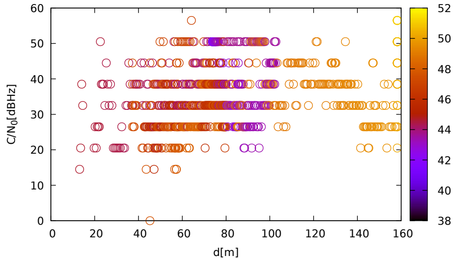
C/N 0 vs distance (LeicaGS15 at C 2 for G03 at L2)
