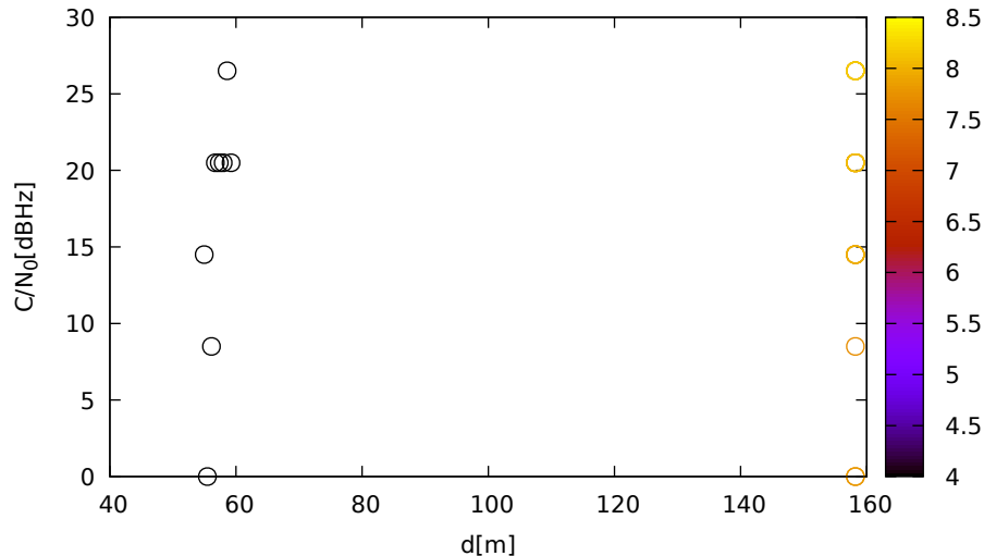
C/N 0 vs distance (LeicaGS15 at C 2 for G04 at L2)
