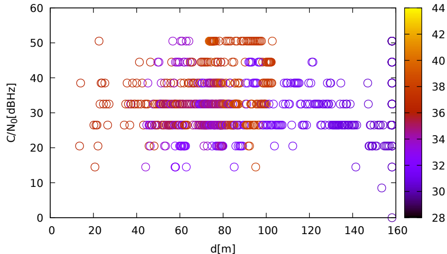
C/N 0 vs distance (LeicaGS15 at C 2 for G08 at L2)
