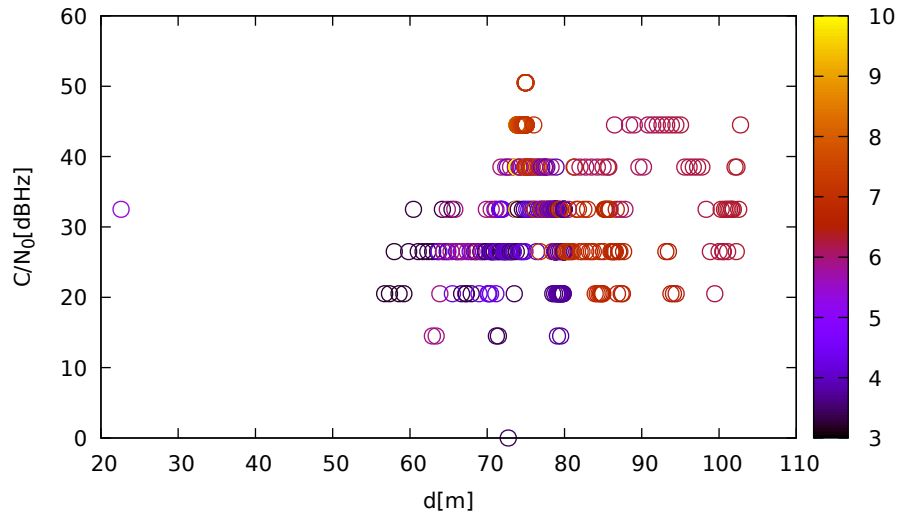
C/N 0 vs distance (LeicaGS15 at C 2 for G10 at L2)
