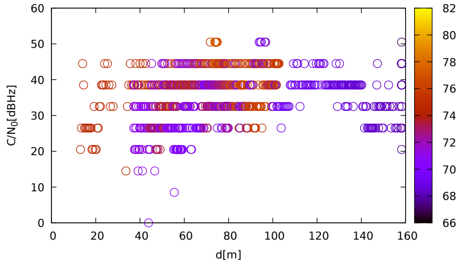
C/N 0 vs distance (LeicaGS15 at C 2 for G11 at L2)
