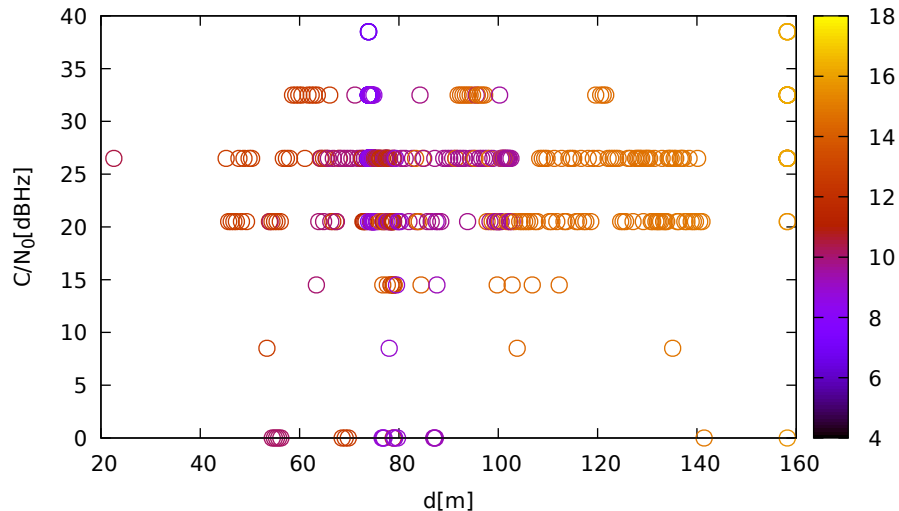
C/N 0 vs distance (LeicaGS15 at C 2 for G17 at L2)
