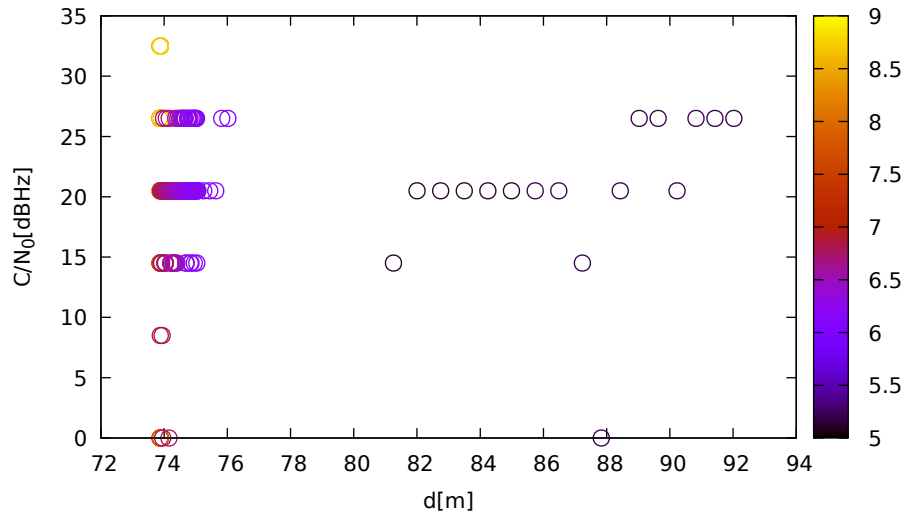
C/N 0 vs distance (LeicaGS15 at C 2 for G21 at L2)
