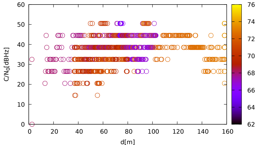
C/N 0 vs distance (LeicaGS15 at C 2 for G22 at L2)
