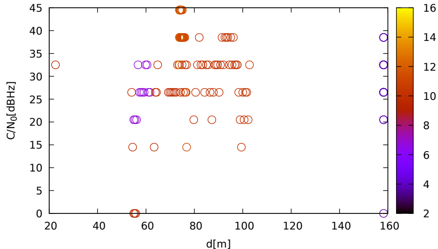
C/N 0 vs distance (LeicaGS15 at C 2 for G27 at L2)
