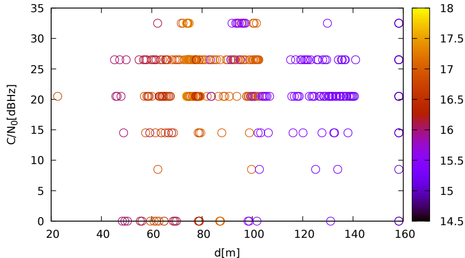
C/N 0 vs distance (LeicaGS15 at C 2 for G28 at L2)
