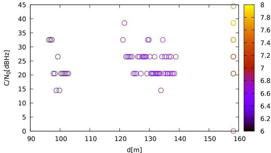
C/N 0 vs distance (LeicaGS15 at C 2 for G31 at L2)
