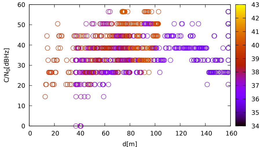
C/N 0 vs distance (LeicaGS15 at C 2 for G32 at L2)
