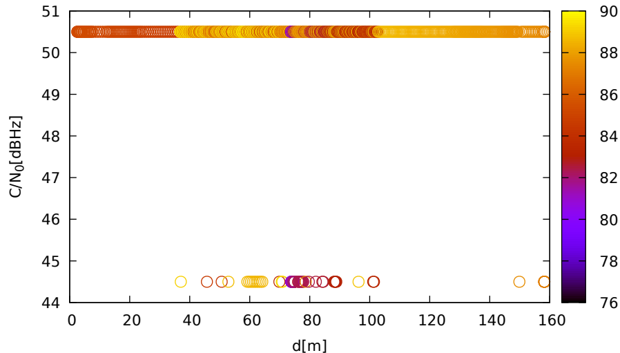
C/N 0 vs distance (LeicaGS15 at C 2 for R07 at L2)
