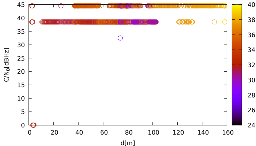
C/N 0 vs distance (LeicaGS15 at C 2 for R08 at L2)
