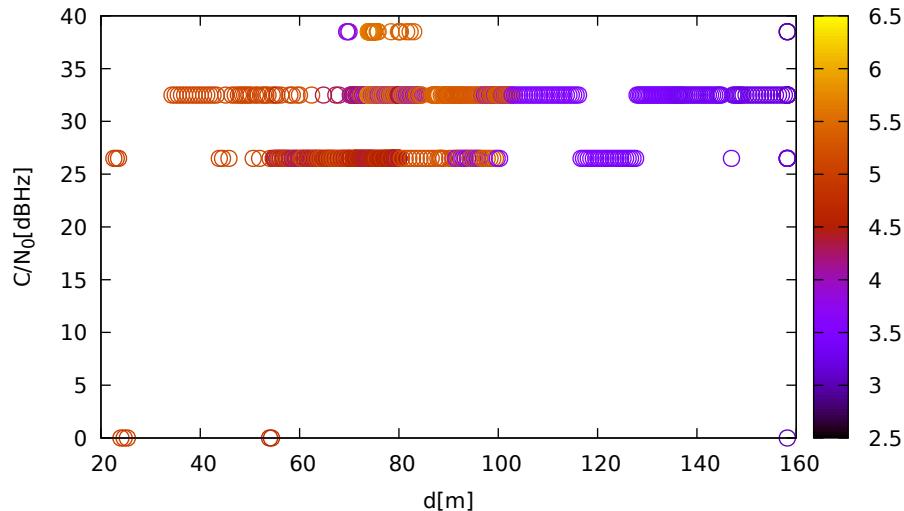
C/N 0 vs distance (LeicaGS15 at C 2 for R14 at L2)
