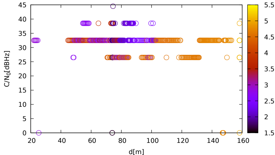
C/N 0 vs distance (LeicaGS15 at C 2 for R15 at L2)
