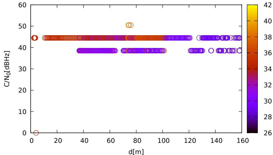
C/N 0 vs distance (LeicaGS15 at C 2 for R21 at L2)
