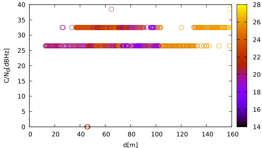
C/N 0 vs distance (LeicaGS15 at C 2 for R23 at L2)
