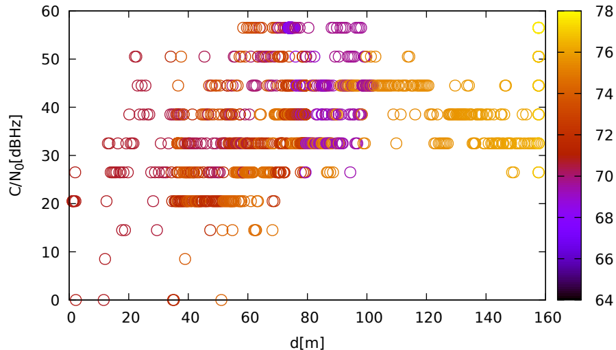
C/N 0 vs distance (LeicaGS18 at C 2 for G01 at L2)
