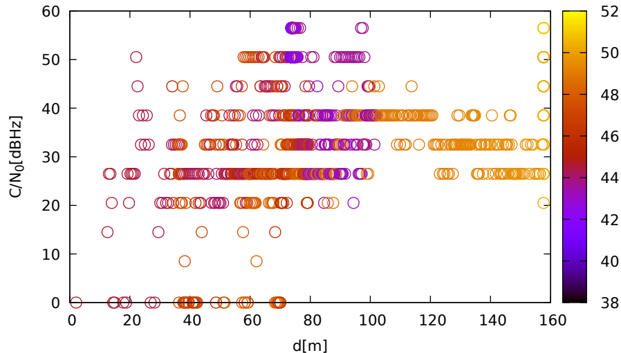
C/N 0 vs distance (LeicaGS18 at C 2 for G03 at L2)
