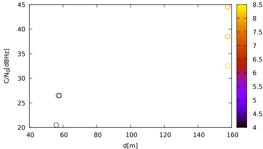
C/N 0 vs distance (LeicaGS18 at C 2 for G04 at L2)
