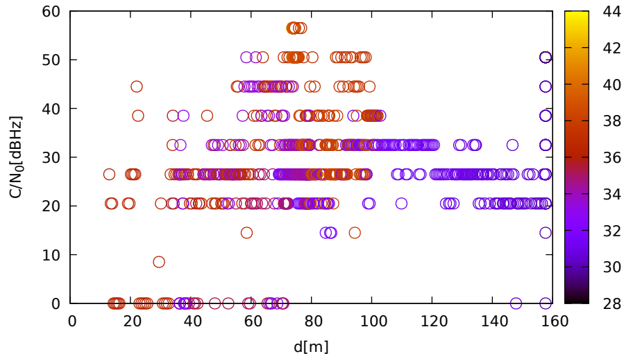
C/N 0 vs distance (LeicaGS18 at C 2 for G08 at L2)
