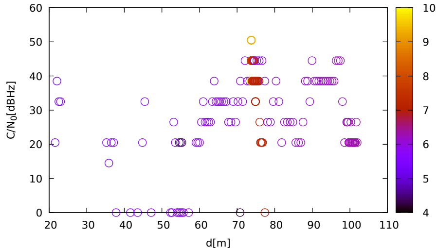
C/N 0 vs distance (LeicaGS18 at C 2 for G10 at L2)
