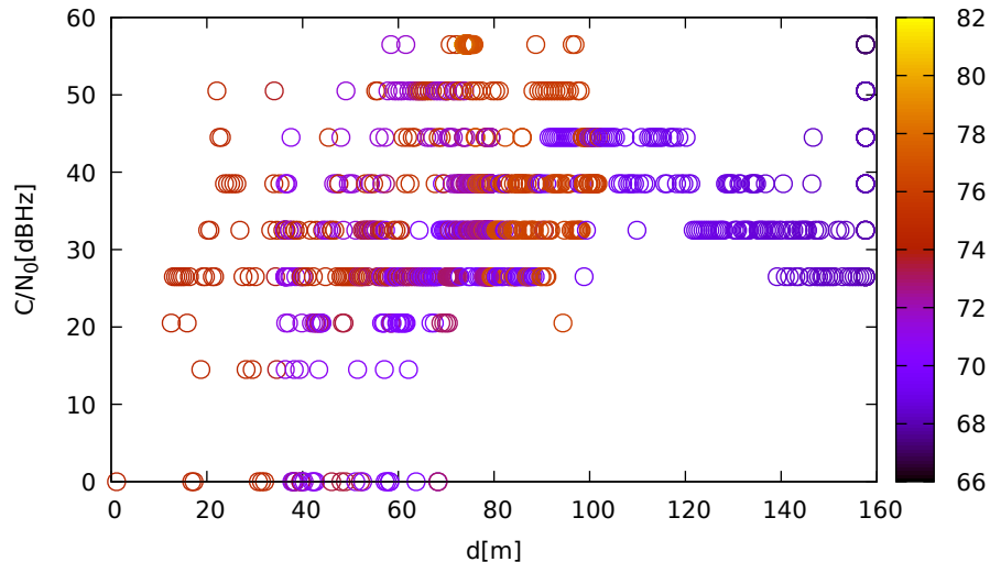
C/N 0 vs distance (LeicaGS18 at C 2 for G11 at L2)
