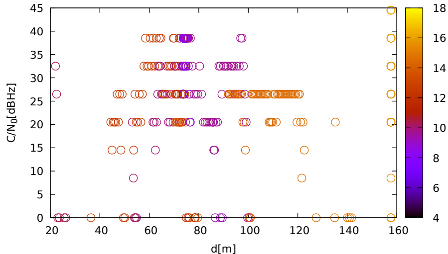
C/N 0 vs distance (LeicaGS18 at C 2 for G17 at L2)
