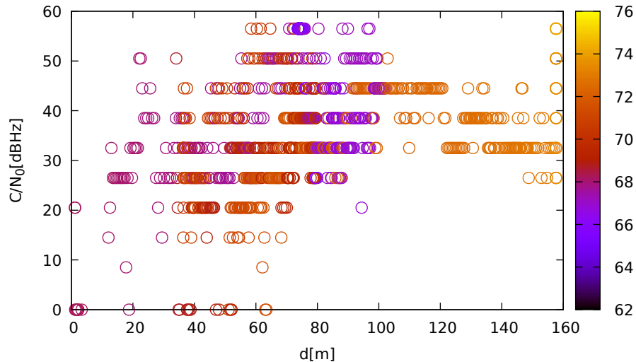
C/N 0 vs distance (LeicaGS18 at C 2 for G22 at L2)
